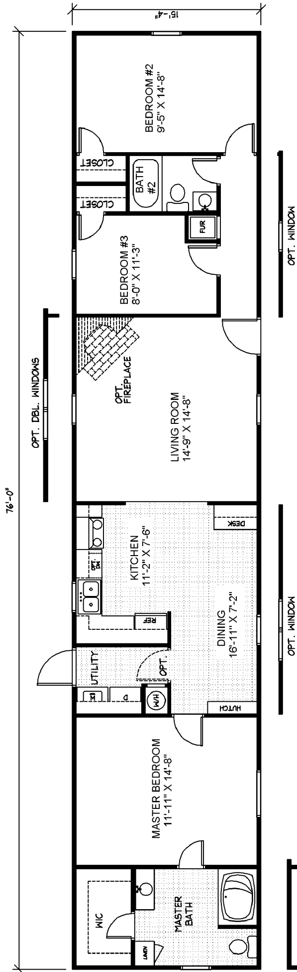
FLOOR PLAN SQUARE FEET = 1165
